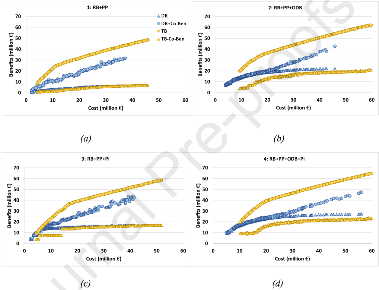
Figure 5. Pareto fronts obtained for damage minimisation (DR) and the result adding co-benefits (DR+Co_Ben), and total benefits maximisation (TB) and the result removing co-benefits (TB-Co_Ben).
