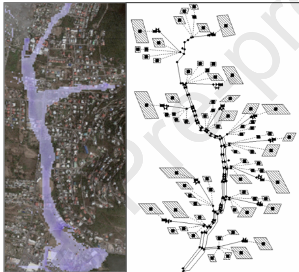
Figure 2. 1D-2D flood modelling result (left) and 1D-1D model representation (right)
